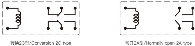
转换2C型/Conversion 2C type
